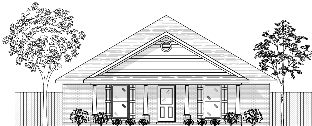
ELEVATION (B)
