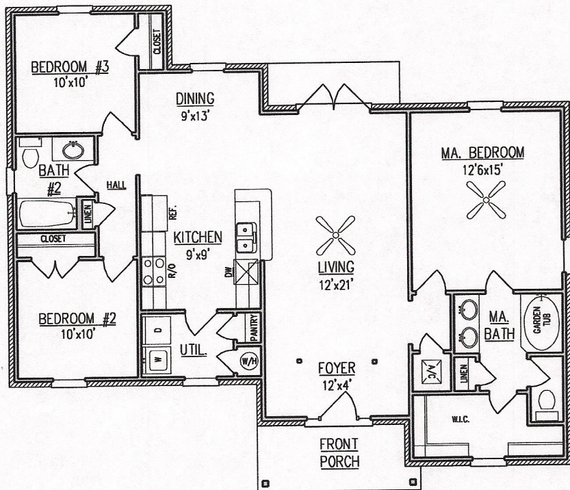
FLOOR PLAN
