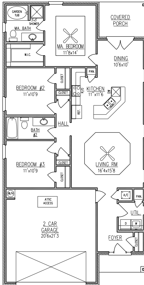
FLOOR PLAN
