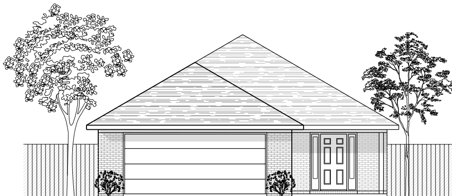
ELEVATION (A)
